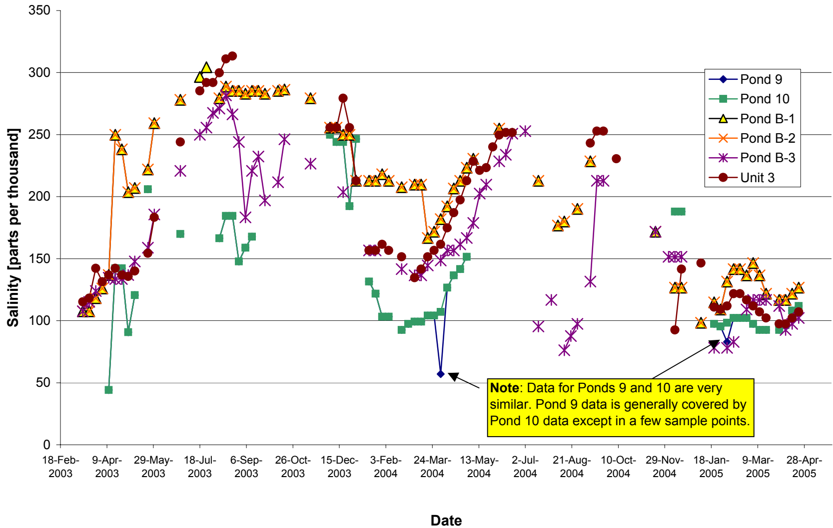
Figure 4-1. Napa Plant Site Pickle Pond Salinity Data
